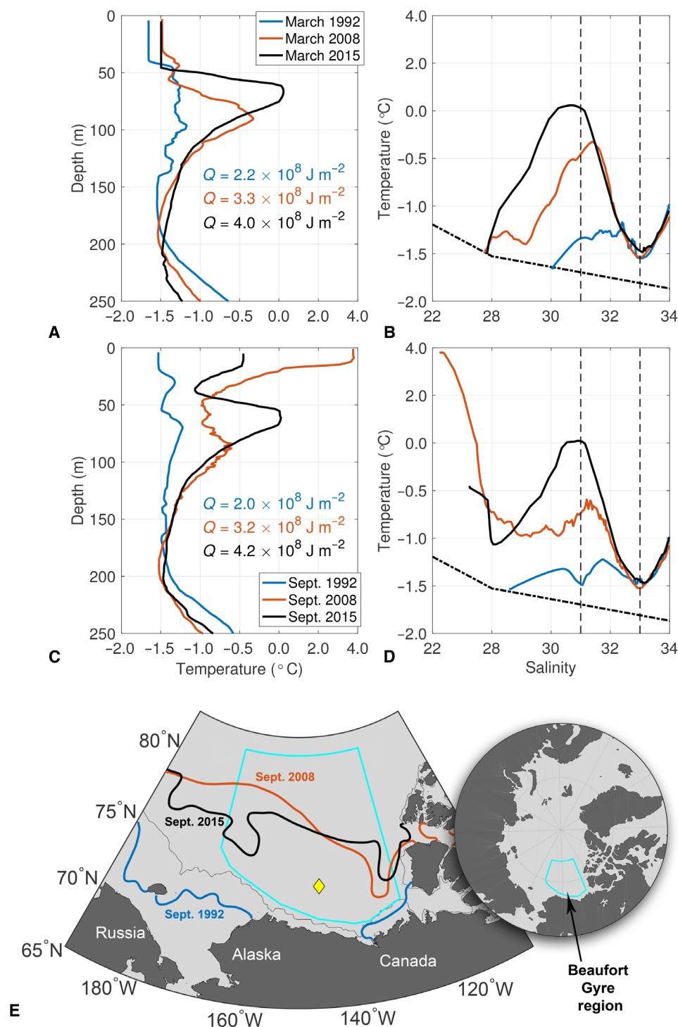
Fig. 1. Temperature and salinity in the BG. (A) Temperature and depth profiles in March 1992, 2008, and 2015 and (B) the same profiles on the temperature-salinity plane. The dashed-dotted black line indicates the freezing temperature at zero pressure, and the vertical dashed lines mark S = 31 and S = 33 . (C) and (D) are the same, with the profiles being from September 1992, 2008, and 2015. Heat content ( Q , \text{J m}^{-2} ) relative to the freezing temperature integrated between the isohalines S = 31 and S = 33 is shown in (A) and (C) for the profiles plotted. All profiles are in the vicinity of the diamond shown in the regional map (E), which was free of sea ice in September 2008 and 2015, and ice covered for the other profiles (contours indicate the monthly sea ice edge; 15% concentration); the cyan boundary delineates the BG region.
