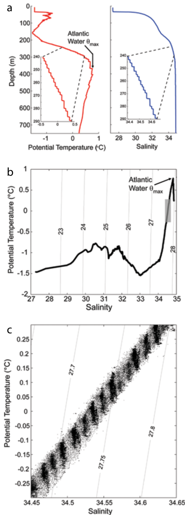
Figure 8. (a) Ice-Tethered Profiler (ITP) profiles of potential temperature and salinity in the Canada Basin. The insets with expanded scales show the double-diffusive staircase. In these profiles, the Arctic surface mixed layer extends to about 40 m depth, with shelf-modified Pacific water from Bering Strait immediately below. A strong thermocline denotes the boundary between the upper waters and the Atlantic Water. Within the thermocline, temperature and salinity increase monotonically with depth, a necessary condition for double-diffusive layering. (b) The corresponding potential temperature/salinity curve and lines of constant potential density anomaly (referenced to the surface). (c) Discrete potential temperature/salinity values from 1000 ITP profiles in the Canada Basin ( \sim 0.25 m vertical resolution), and lines of constant potential density anomaly (referenced to the surface). The region in potential temperature/salinity space is shown by the grey box in panel (b). Staircase mixed-layer properties tend to group along lines in potential temperature/salinity space; Timmermans et al. (2008a) show that individual mixed-layers are coherent for at least 800 km across the basin and persist for several years. After Timmermans et al. (2008b)
