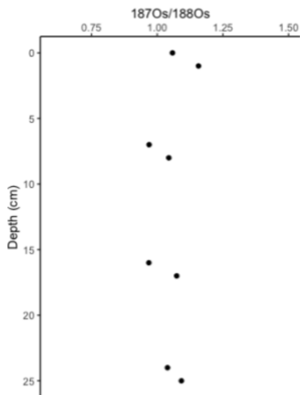
Figure 6. Depth profile of ^{187}\text{Os}/^{188}\text{Os} isotopic composition of the FOAM sediment core from the Long Island Sound.
