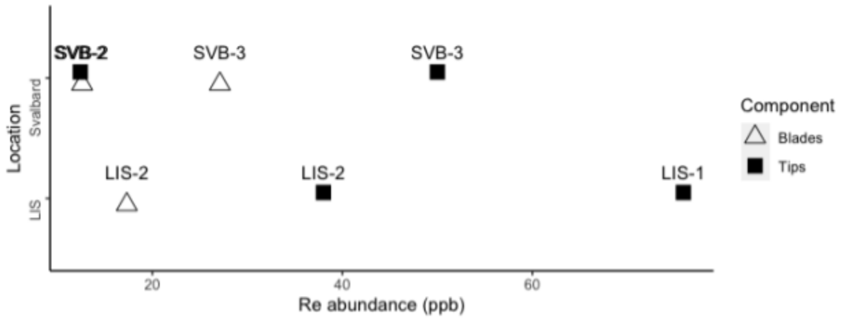
Figure 7. Re abundances for macro-algae samples plotted by study site and seaweed component.
